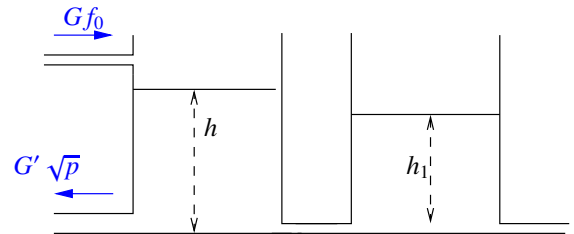
Fig. 5. We amplify the input flow f_0 through a large gain G and we apply a large negative feedback by employing a large output pipe with output flow G'\sqrt{p} .
