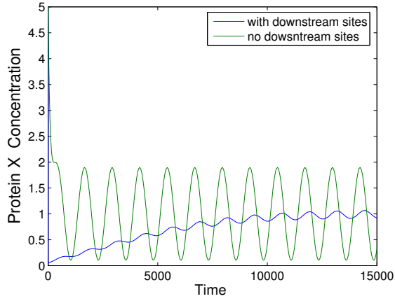
Fig. 4. Simulation results for the system in equations (3). In the plot, k(t) = 0.01(1 + \sin(\omega t)) with \omega = 0.005 , k_{on} = 10 , k_{off} = 10 , \delta = 0.01 , p_{TOT} = 100 , X(0) = 5 . The amount of downstream binding sites is large compared to X(0) as it occurs in synthetic systems in which these sites are present in high copy-number plasmids. Time is in minutes. The green plot represents X(t) originating by the isolated system in equations (2), while the blue plot represents X(t) obtained by the interconnected system of equation (3). Both transient and permanent behaviors are different.
