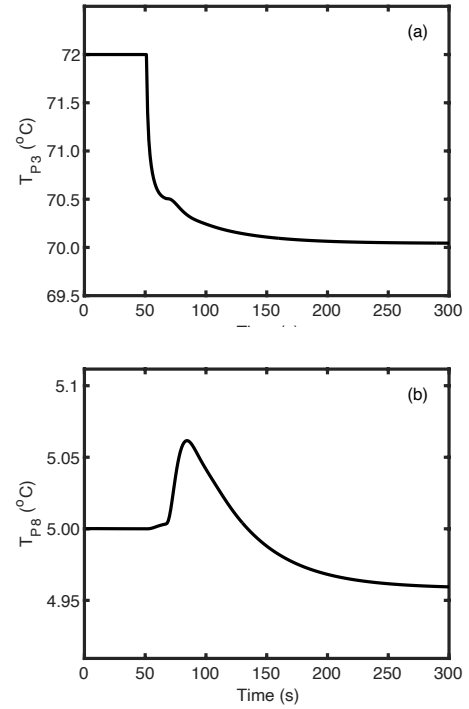
Figure 2. Milk temperature at the exit of the heater (a) and at the exit of cooler (b) after a step change of the hot water temperature equal to -2°C from the nominal set-point.
