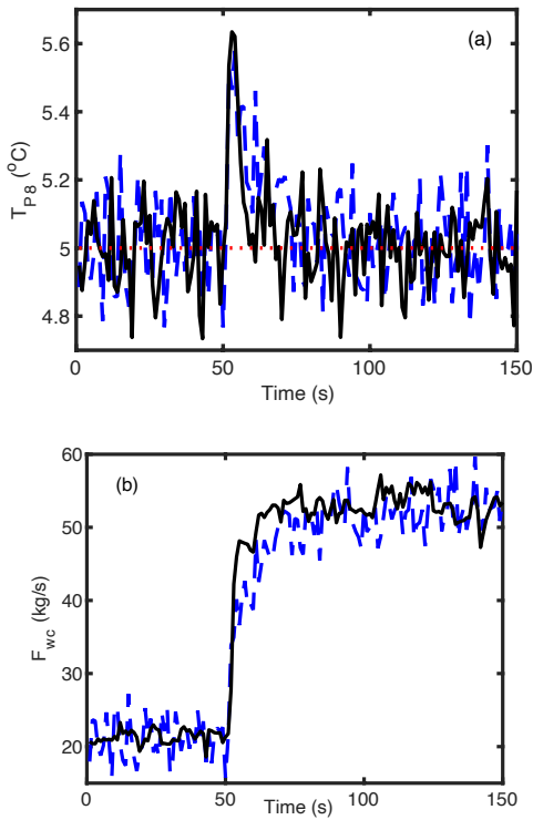
Figure 6. Temperature T_{P8} (a) and flowrate F_{wc} (b) responses when T_{h1} varies from 75^{\circ}\text{C} to 73^{\circ}\text{C} , T_{c1} from 2.5^{\circ}\text{C} to 4^{\circ}\text{C} . NMPC (black continuous line), PI (dashed blue line) and set-point (red dotted line).
