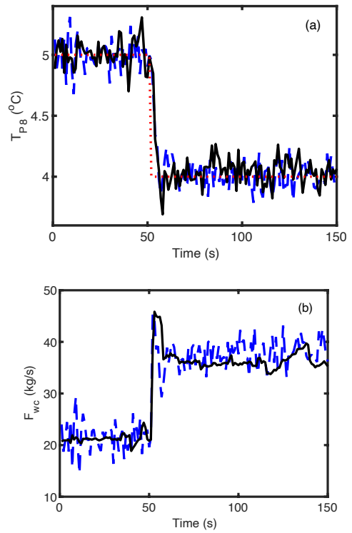
Figure 8. Temperature T_{P8} (a) and flowrate F_{wc} (b) responses for set-point change of T_{P8} from 5^{\circ}\text{C} to 4^{\circ}\text{C} . NMPC (black continuous line), PI (dashed blue line) and set-point (red dotted line).
