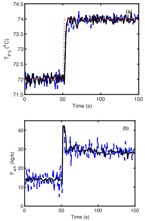
Figure 7. Temperature T_{P3} (a) and flowrate F_{wh} (b) responses for set-point change from 72^{\circ}\text{C} to 74^{\circ}\text{C} . NMPC (black continuous line), PI (dashed blue line) and set-point (red dotted line).
