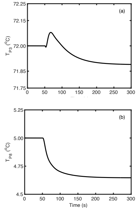
Figure 3. Milk temperature at the exit of the heater (a) and at the exit of cooler (b) after a step change of the inlet milk temperature equal to -2°C from the nominal set-point.
