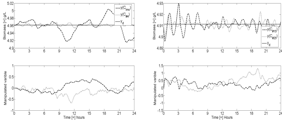
(a) Noisy simulation of the closed loop system at dilution rate 0.7 \text{ h}^{-1} with the initial IMC controller and the fourth iterate from the IFT tuning method.
