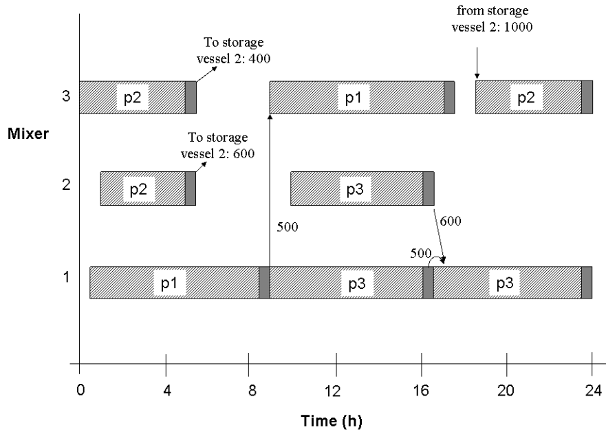
Figure 1. Schedule for first example
