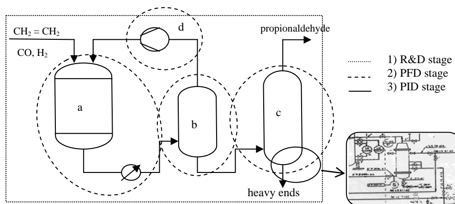
Figure 1. Utilization of Evaluation Levels on the Different Stage Methods in the Case Study Process; 1) process step at R&D stage, 2) standard modules of the predesign stage, 3) piping details at basic engineering stage (a=reactor, b=flash, c=distillation system, d=compressor)
