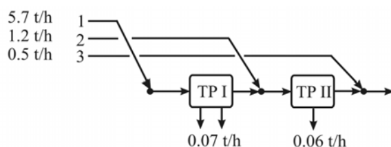
Fig. 1. Final design for glass container factory case study.
