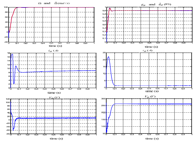
Fig. 1. Responses of the IM in un-faulty mode
