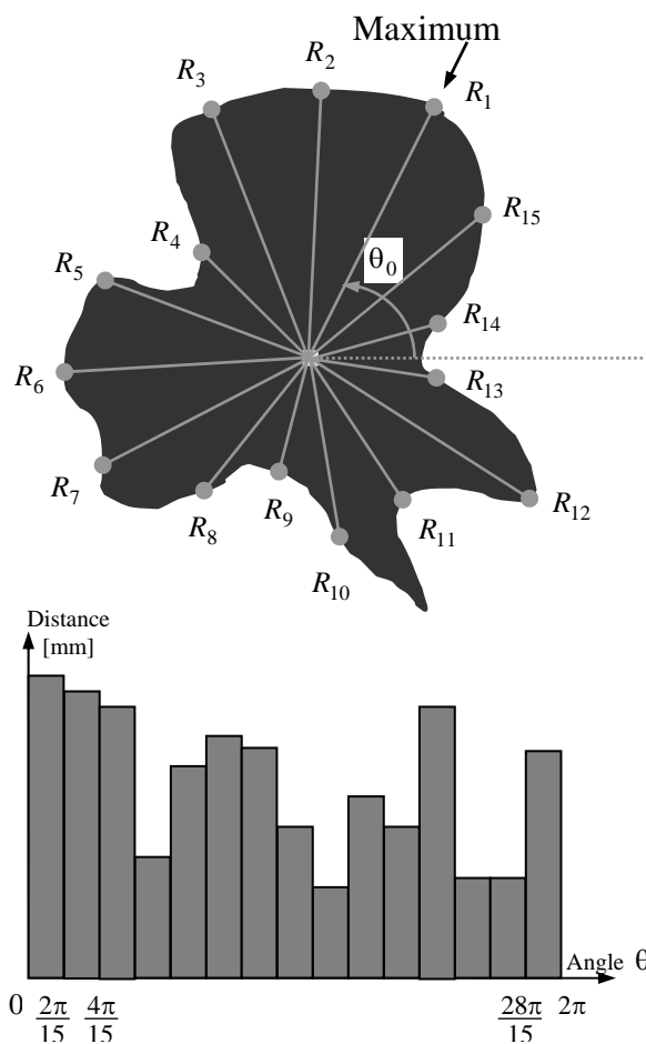
Fig. 2 Angular radii signature of a shape. A 15-element vector [R_1, R_2, \dots, R_{15}] is defined, where R_i, i = 1, \dots, 15 is the distance from the centroid to the edge of the blob, measured at an angle of (\theta_0 + 24i) degrees, and \theta_0 is the orientation derived from the greatest radius, R_1 .
