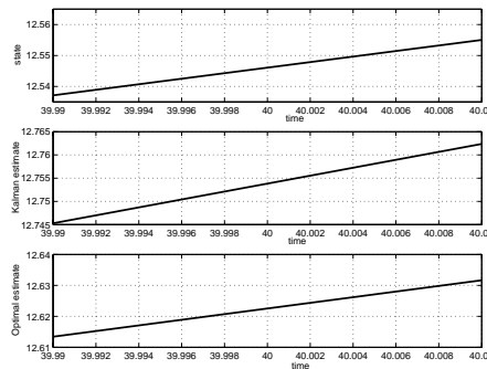
Figure 2. Graphs of the reference state variable x(t) and the estimates m_K(t) and m(t) around the reference time point T = 40 .
