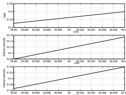
Figure 3. Graphs of the reference state variable x(t) and the estimates m_K(t) and m(t) around the reference time point T = 60 .
