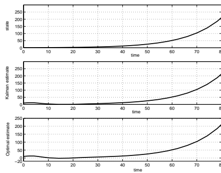
Figure 1. Graphs of the reference state variable x(t) and the estimates m_K(t) and m(t) on the entire simulation interval [0, 80] .
