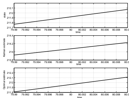
Figure 4. Graphs of the reference state variable x(t) and the estimates m_K(t) and m(t) around the reference time point T = 80 .
