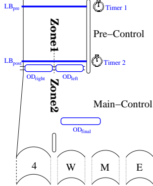
Fig. 3. Layout of the northern tunnel entrance
