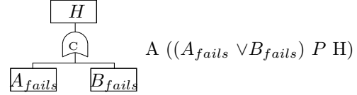
Fig. 2. Incorrect fault tree
