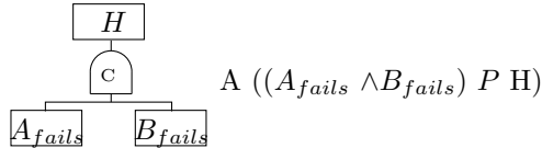
Fig. 1. Fault tree AND-gate and formalization
