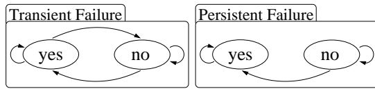
Fig. 4. Failure automata for transient and persistent failures
