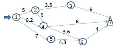
Fig. 1. A 7-node network with charging nodes.
