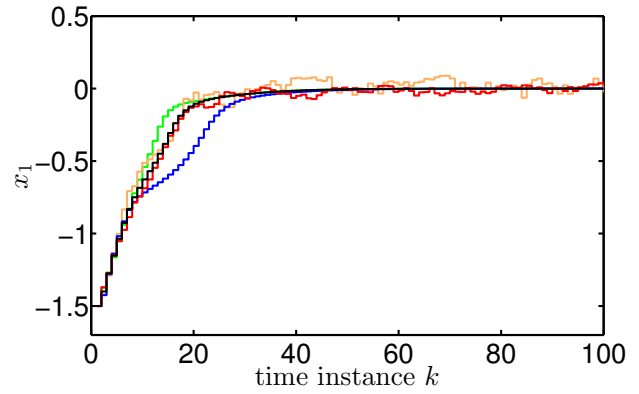
(a) Evolution of the state x_1
