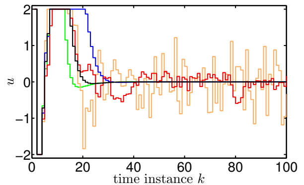
(c) Input signal u
