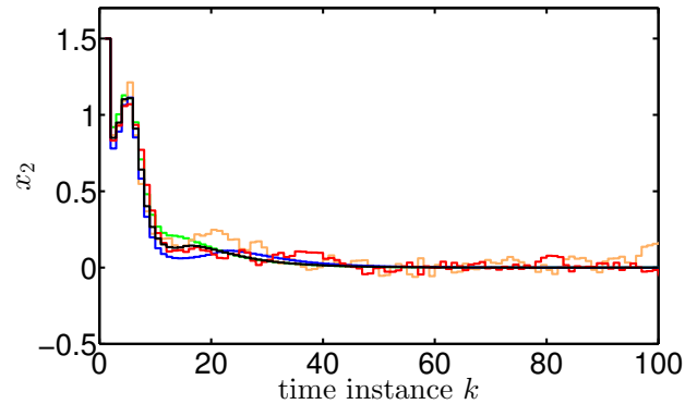
(b) Evolution of the state x_2
