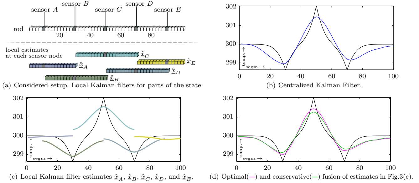
Fig. 3. Temperature profile of rod is to be estimated and is drawn black. A centralized Kalman filter is compared with several local Kalman filters on unequal parts of the state and subsequent fusion.
