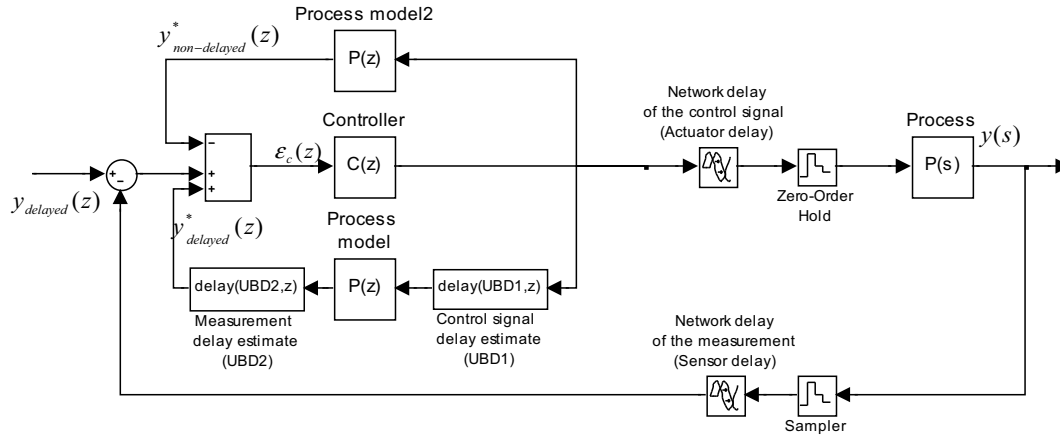
Fig. 4. A Smith predictor scheme for compensation of the network induced delay
