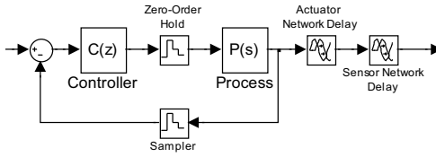
Fig. 5. The equivalent Smith predictor compensation scheme in case the delay is commutative
